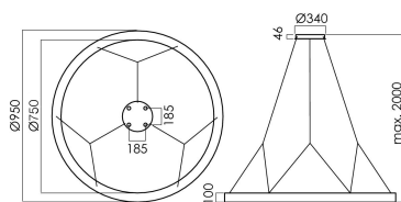
Diameter 950mm
